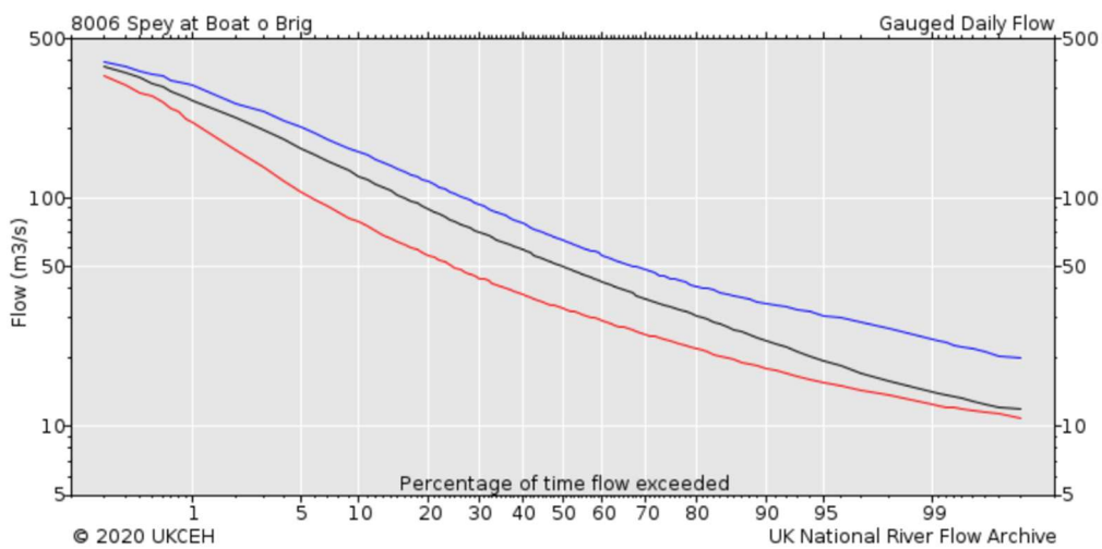
Figure 4.3: Gauging station flow duration curves
