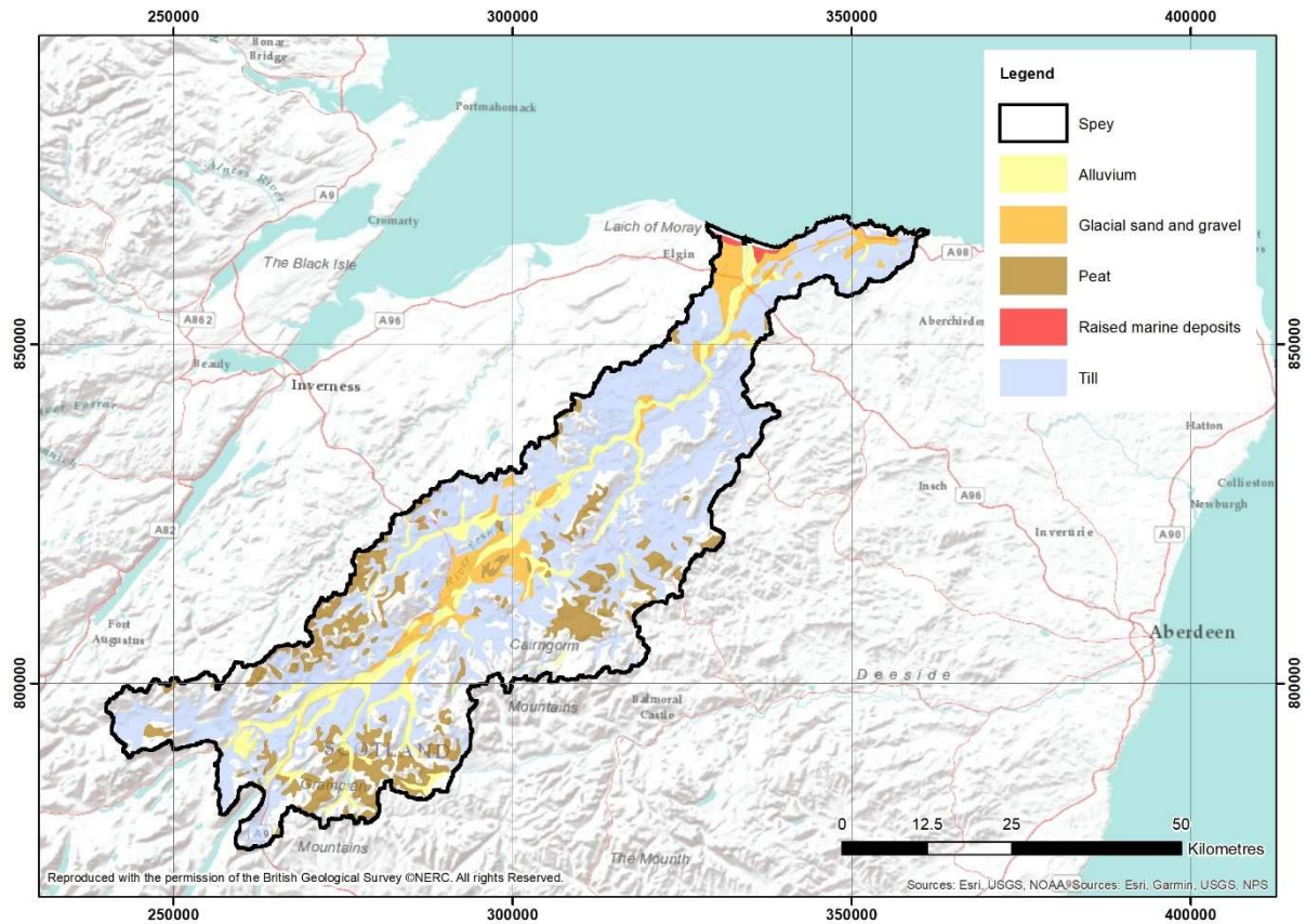
Figure 5.9: Superficial geology deposits within the Spey catchment
