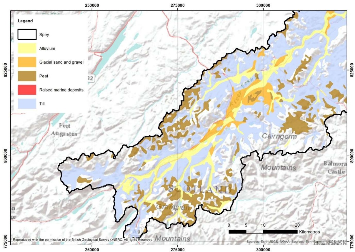
Figure 5.10: Extent of alluvial and glacial deposits within the river valleys of the upper Spey
