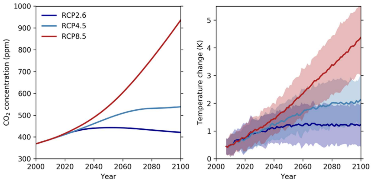
Figure 5.2: Representative Concentration Pathways (RCPs) for future UKCP18 climate scenarios
